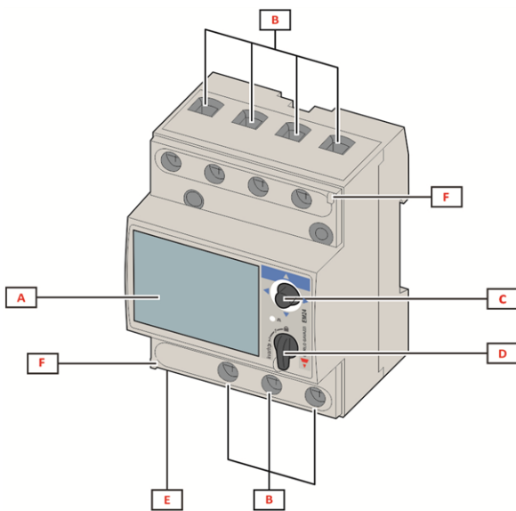
Fig. 1 Direct connection
